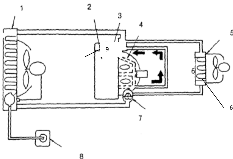
2-rasm. Sovuq dvigatelda suyuqlikni aylanishi:
